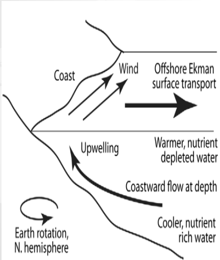
Figure 5.1. Coastal upwelling.
