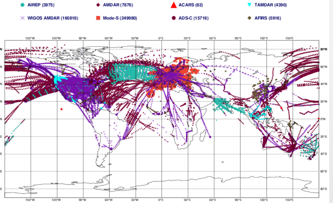
ECMWF data coverage (all observations) - AIRCRAFT 2022011021 to 2022011103 Total number of obs = 448753
